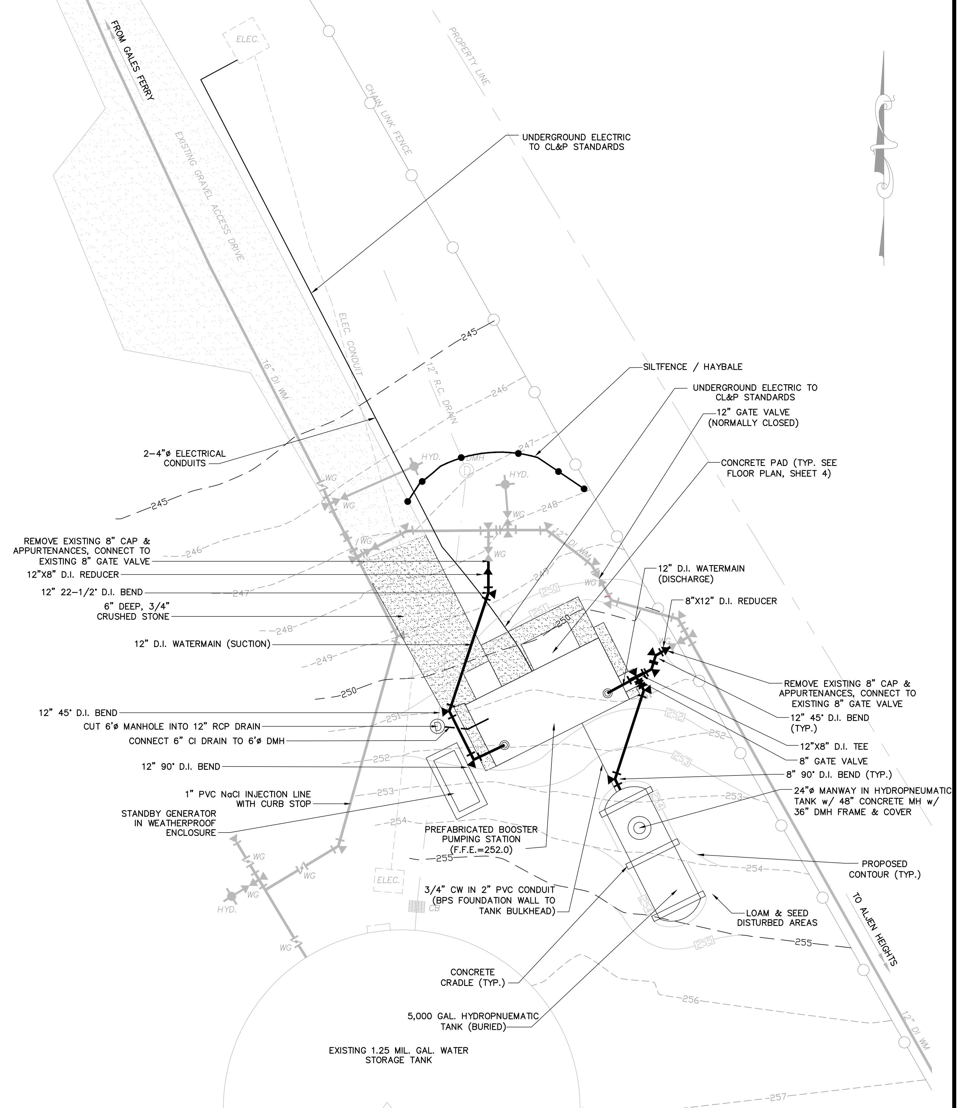
PROPOSED SITE PLAN SCALE: 1" = 10'-0"
