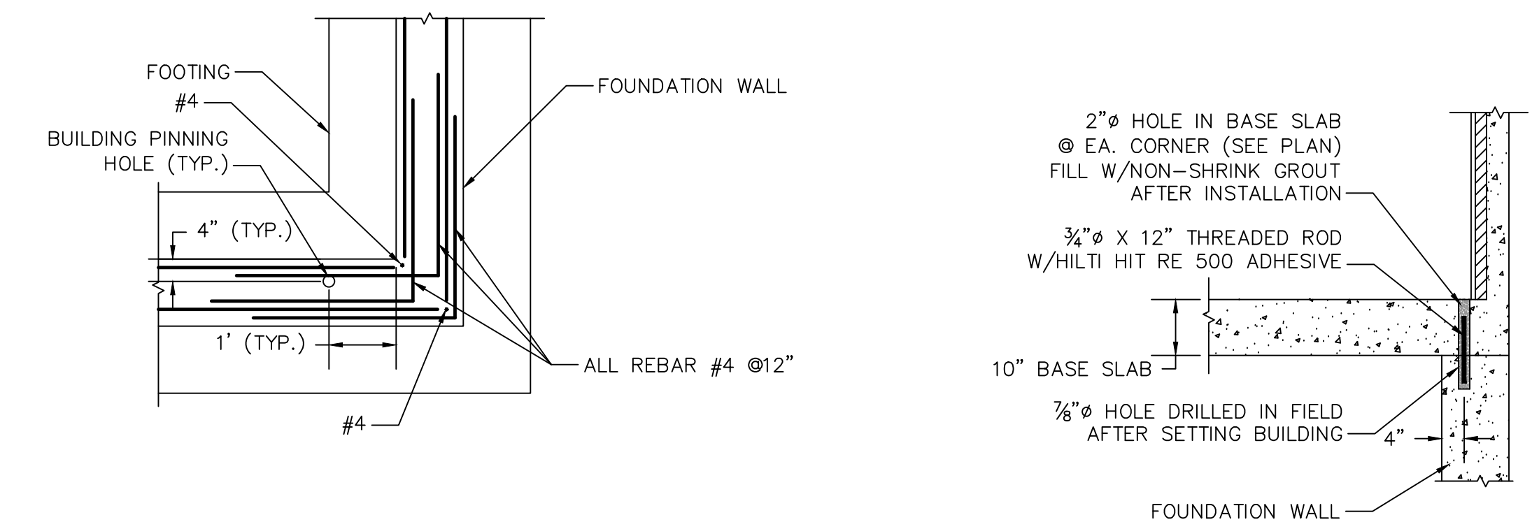
5 CORNER DETAIL SCALE: 1/2" = 1'-0"
